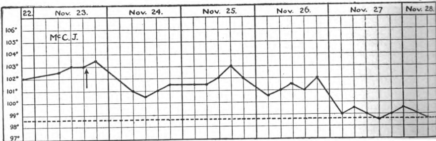
Chart 19.—Temperature curve of donor McC. J.
