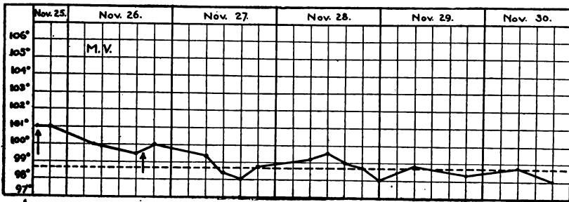
↑ = USED FOR EXPERIMENT. Chart 22.—Temperature curve of donor M. V.
