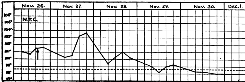
↑ = USED FOR EXPERIMENT. Chart 23.—Temperature curve of donor N. T. C.
