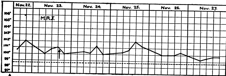
↑ = USED FOR EXPERIMENT. Chart 21.—Temperature curve of donor M. R. J.
