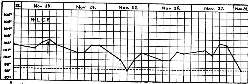
↑ = USED FOR EXPERIMENT. Chart 20.—Temperature curve of donor McL. C. F.
